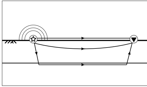
Figure 4.3.: Basic ray paths in the case of a seismic surface source producing ambient acoustic noise for a simple two-layer subsurface model
