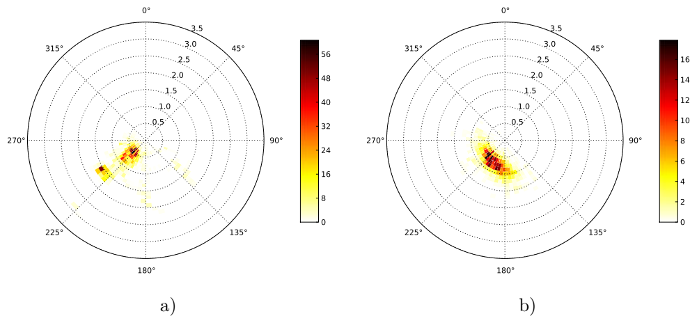
Figure 6.7.: baz-s plot of the signals produced by a nearby motorway observed with the ALBA geophone array: a) unfiltered b) 8 Hz to 12 Hz bandpass-filtered
