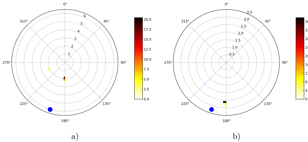
Figure 6.32.: Effects of the PPO window on the array analysis (actual backazimuth indicated by a blue dot): a) KNH geophone array data b) KNH microphone array data
